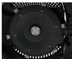
6 cuchillas 6 cutter
